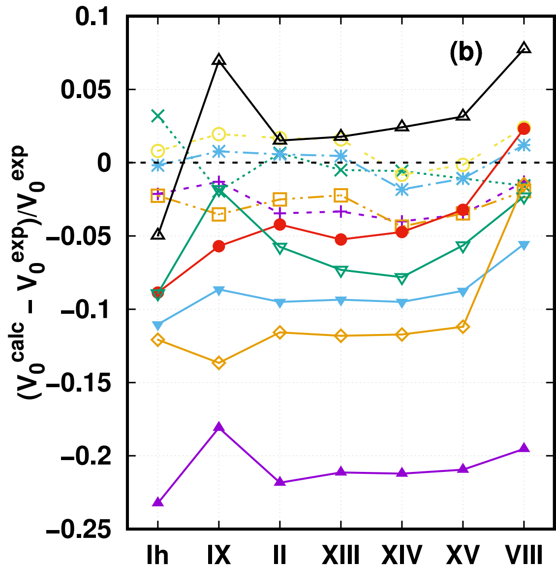
With ZPE
