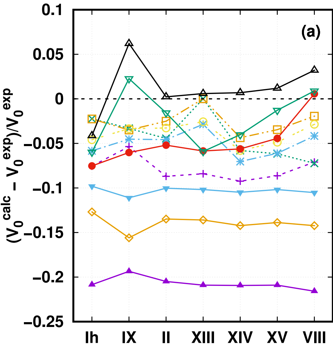
Without ZPE
