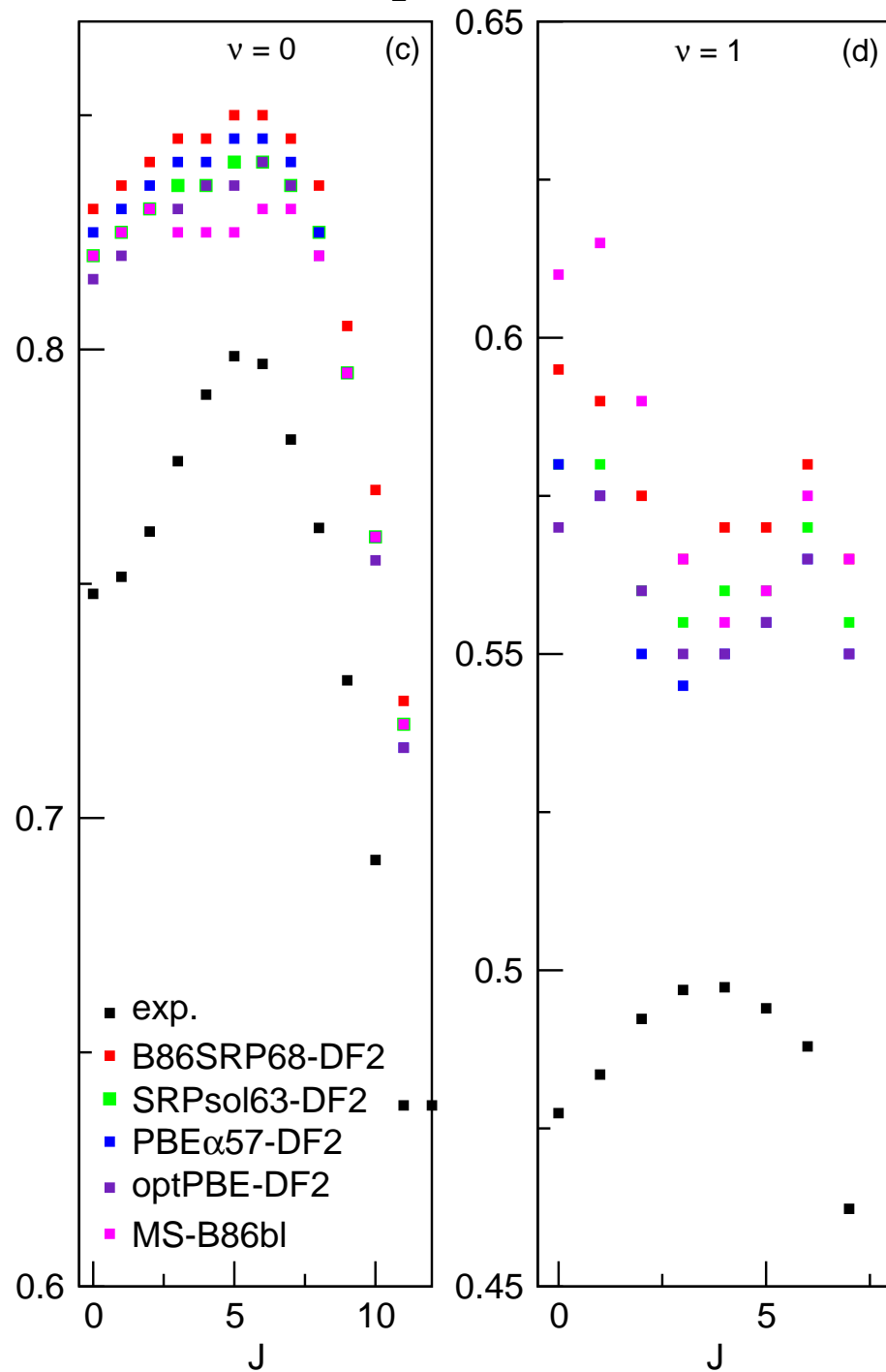
\text{D}_2 + \text{Cu}(111)
