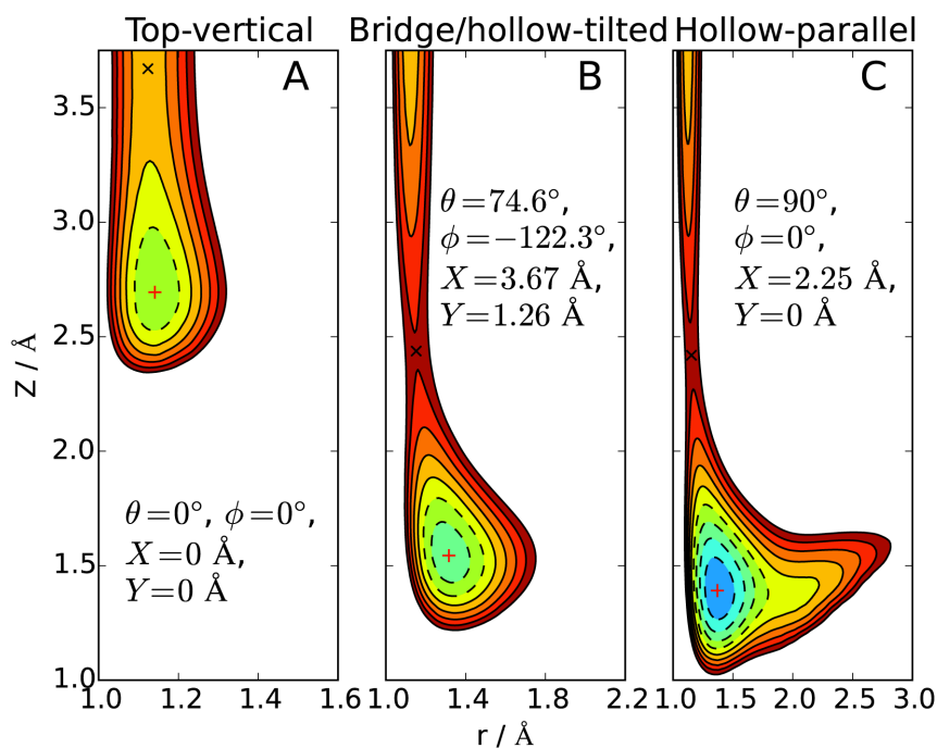
Figure 3: Same as Figure 2, but for RPBE.
