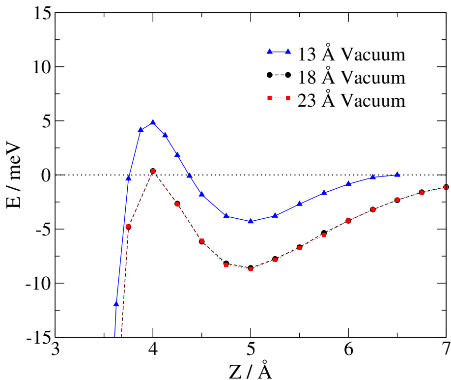
Figure 4: The PBE interaction energy is plotted as a function of Z , using the same equilibrium 5-layer slab to model the W(110) surface, but using different vacuum spaces along the surface normal. The N_2 bond length has been kept equal to the equilibrium value of 1.117 \text{ \AA} . The zero of energy is defined as the energy of the molecule in its equilibrium geometry placed midway between two slabs.
